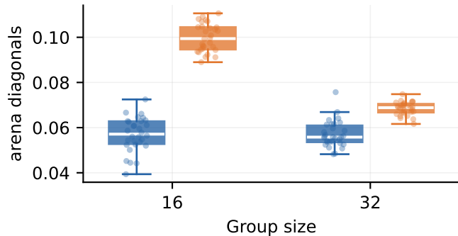
Predator distance
