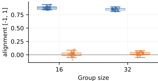
Pursuit alignment
